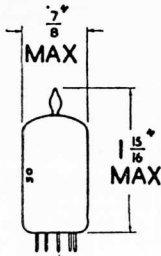
B9A Base
