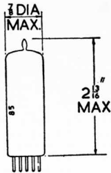
B9A Base
