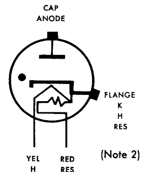
BASING DIAGRAM
