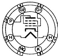
BOTTOM VIEW SHORT INTERMEDIATE SHELL 7 PIN LOW LOSS PHENOLIC
