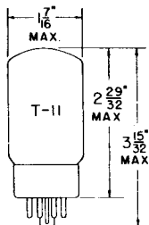
GLASS BULB
