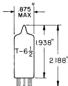
GLASS BULB 9 PIN BASE E9-1 OUTLINE DRAWING JEDEC 6-7
